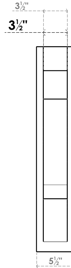
FRONT PROFILE
